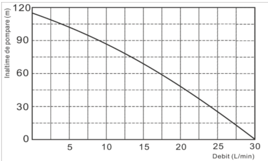
Caracteristica H (m col H 2 O) – Q (l/ min) a pompei 4 QGD 1.8-50-0.5
