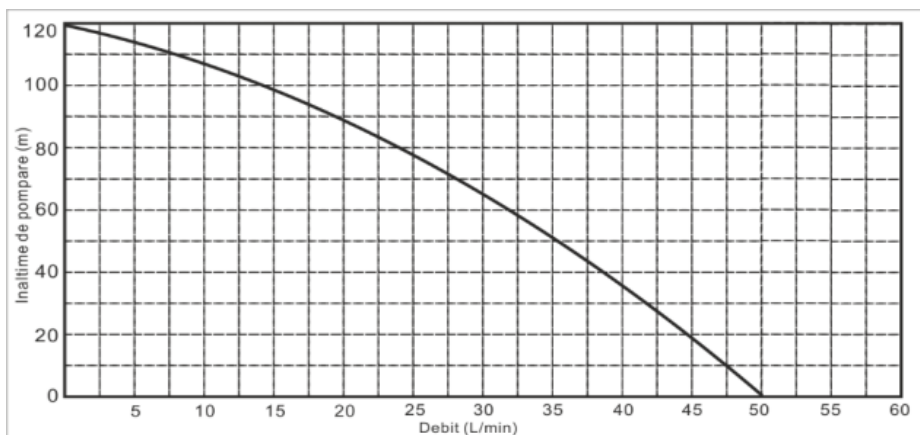
Caracteristica H (m col H 2 O) – Q (l/ min) a pompei 4 QGD 3.5-50-0.75
